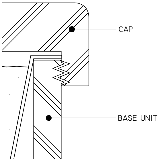
SECTIONAL DETAIL 1 SCALE 1 : 5
